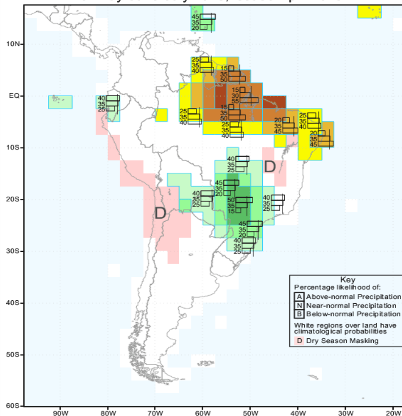
IRI Multi-Model Probability Forecast for Precipitation for May-June-July 2015, Issued April 2015
