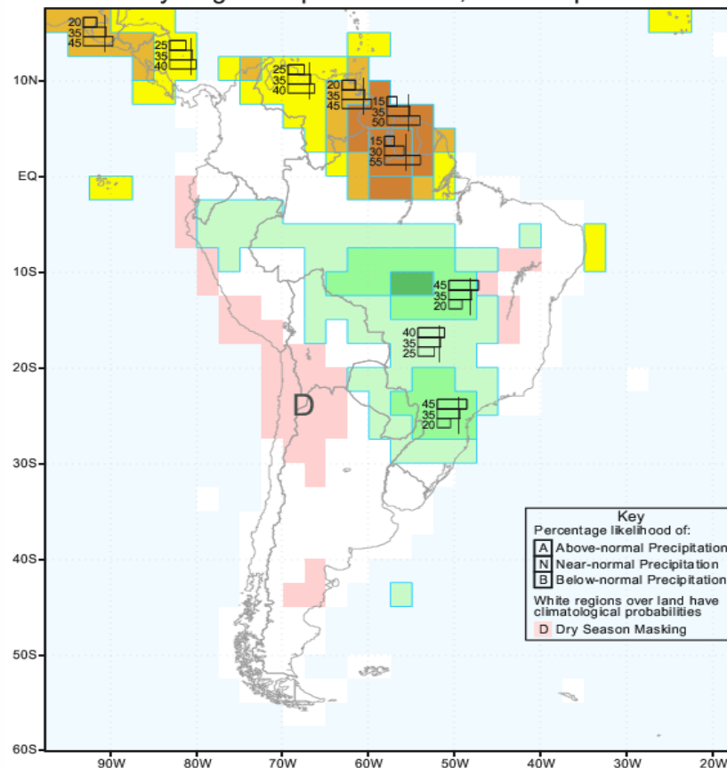
IRI Multi-Model Probability Forecast for Precipitation for July-August-September 2015, Issued April 2015
